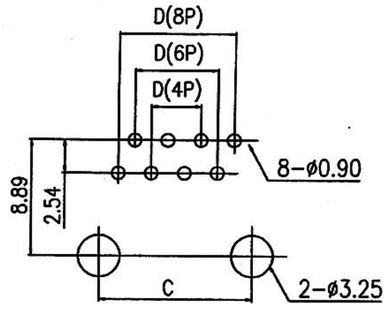
PCB Layout
